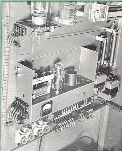
BELOW—Oscillator chassis, completely plug-in and quickly removable in case of urgent servicing. Only one oven shown but two supplied. Crystal change-over switch is on this chassis also. Dust cover has been removed for this illustration.
