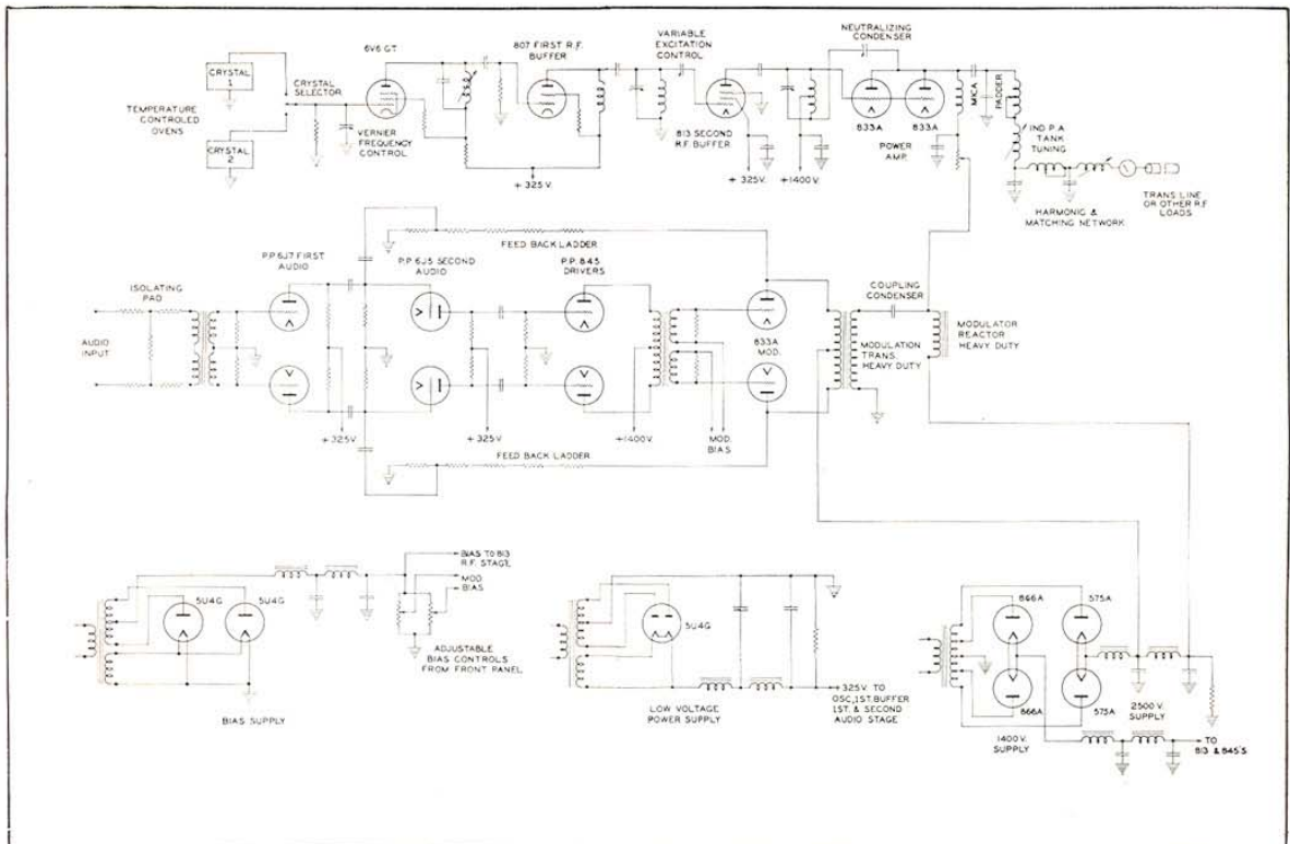
Simplified Schematic BC-1F Transmitter
