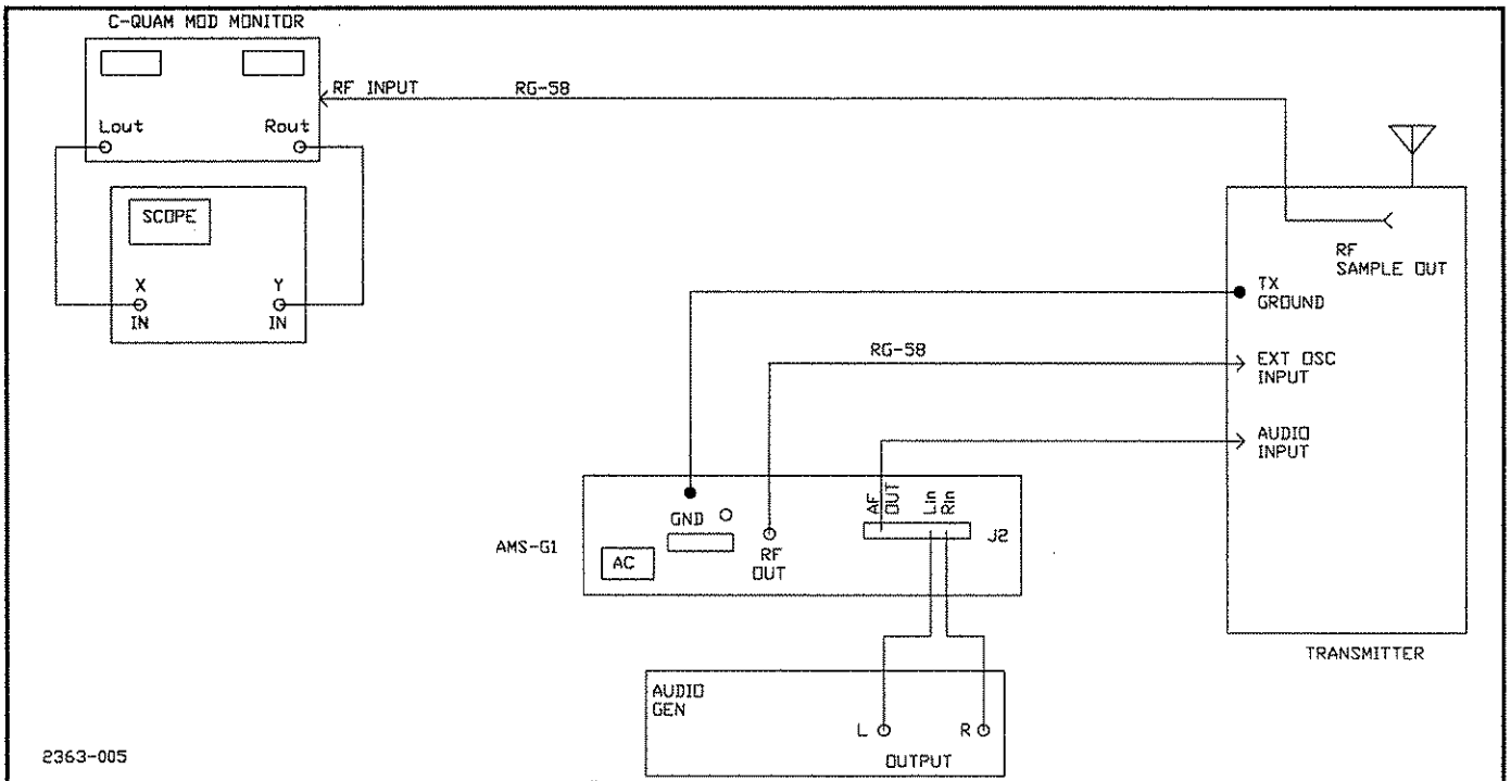
Figure 2-8. AMS-G1 Interconnect Wiring
