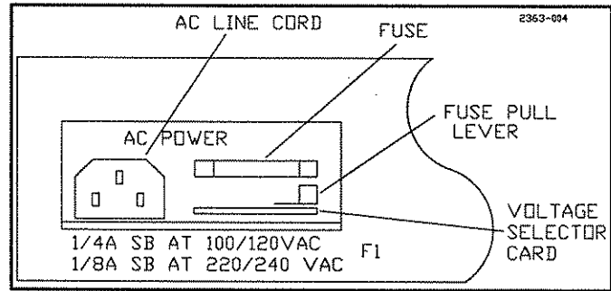
Figure 2-1. AMS-G1 Rear Panel, Left Side
